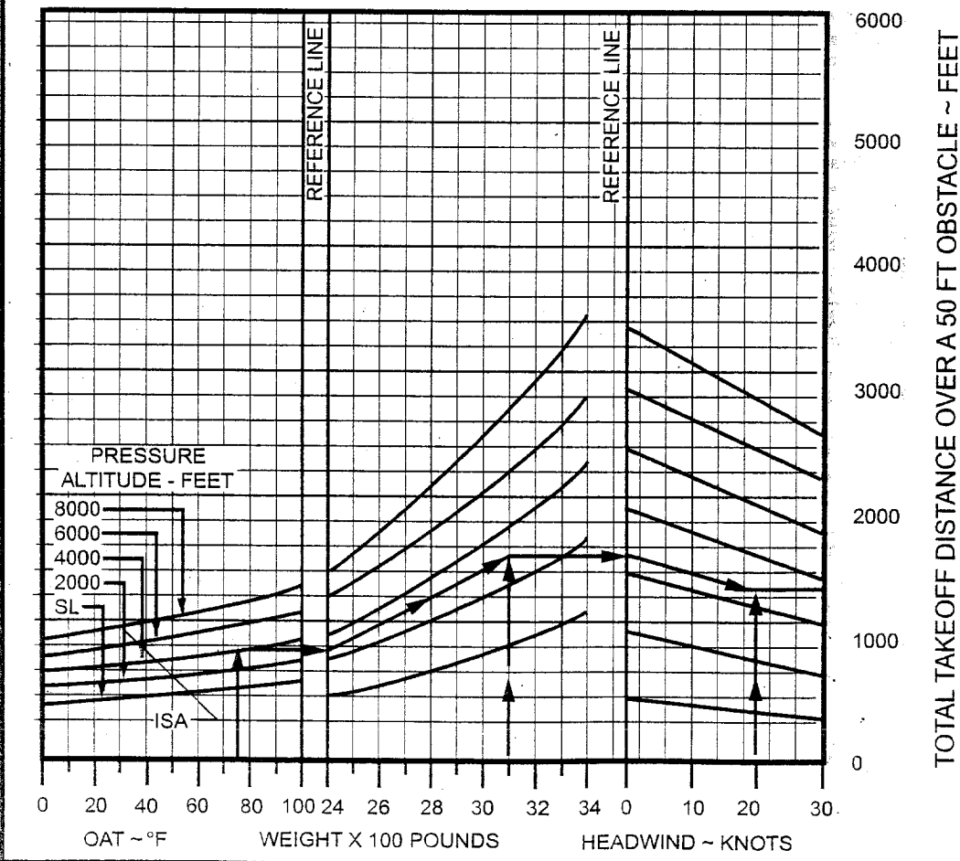
Figure 32. - Obstacle Take-off Chart.
