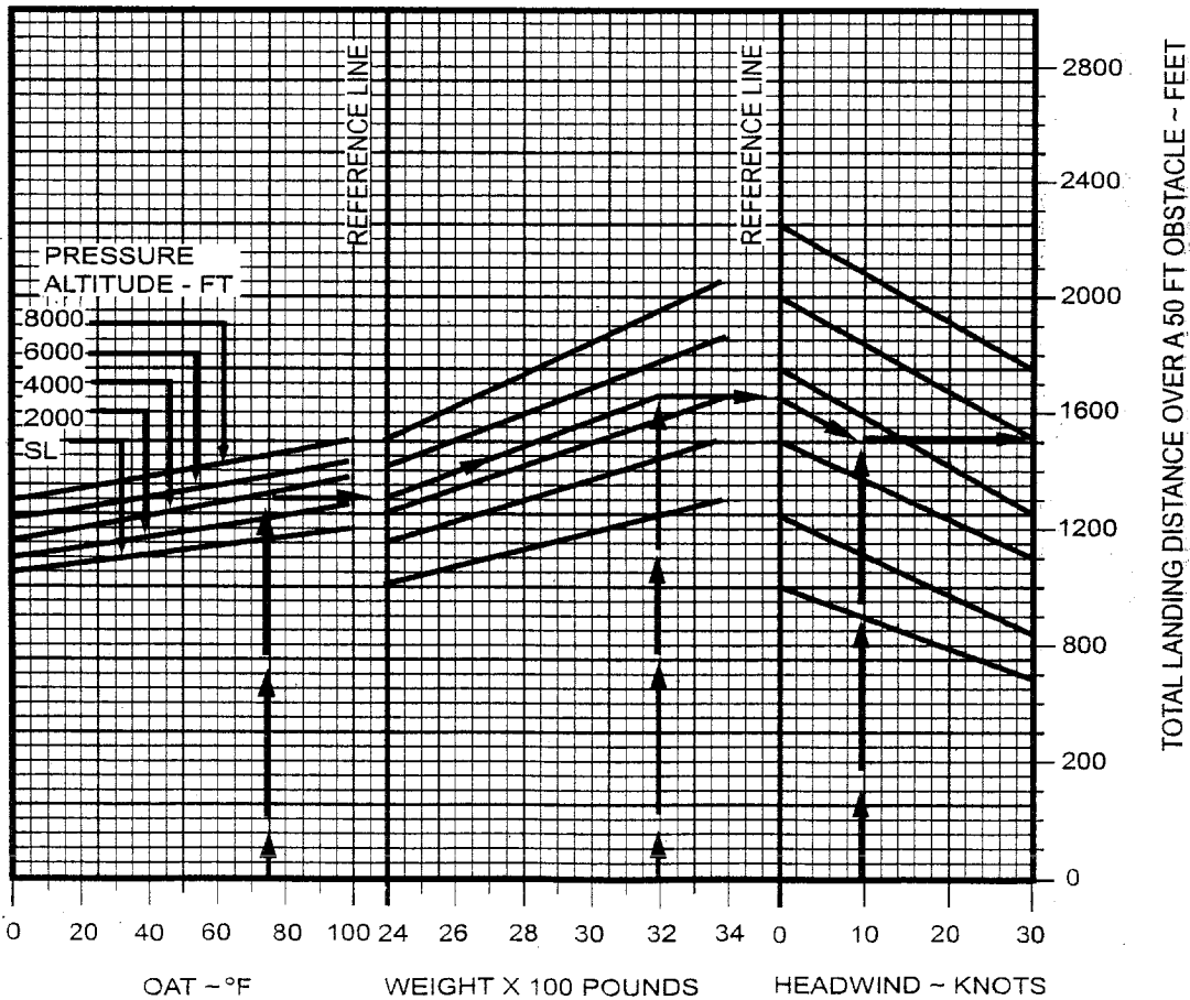
Figure 35. - Normal Landing Chart.
