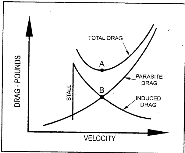
Figure 1. - Drag vs. Speed.
