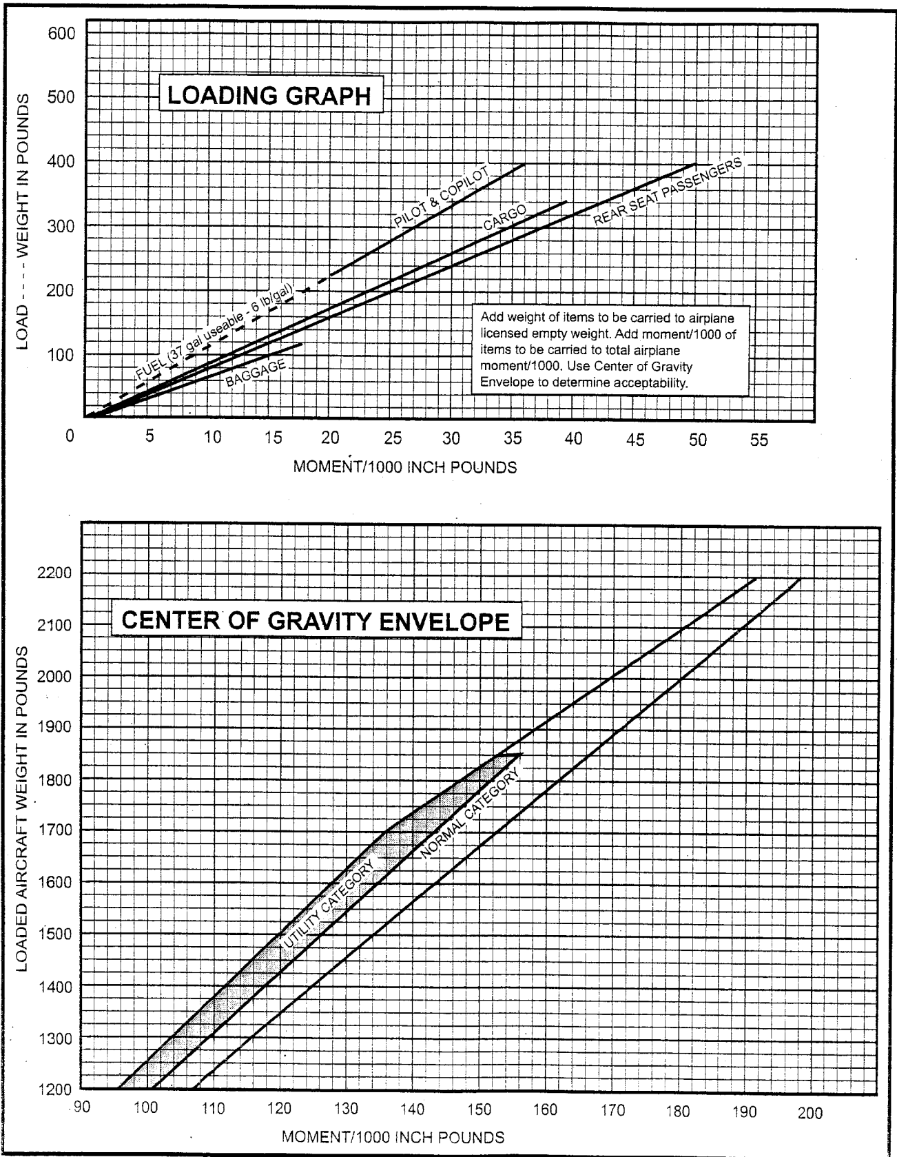
Figure 38. - Loading Graph and Center-of-Gravity Envelope.
