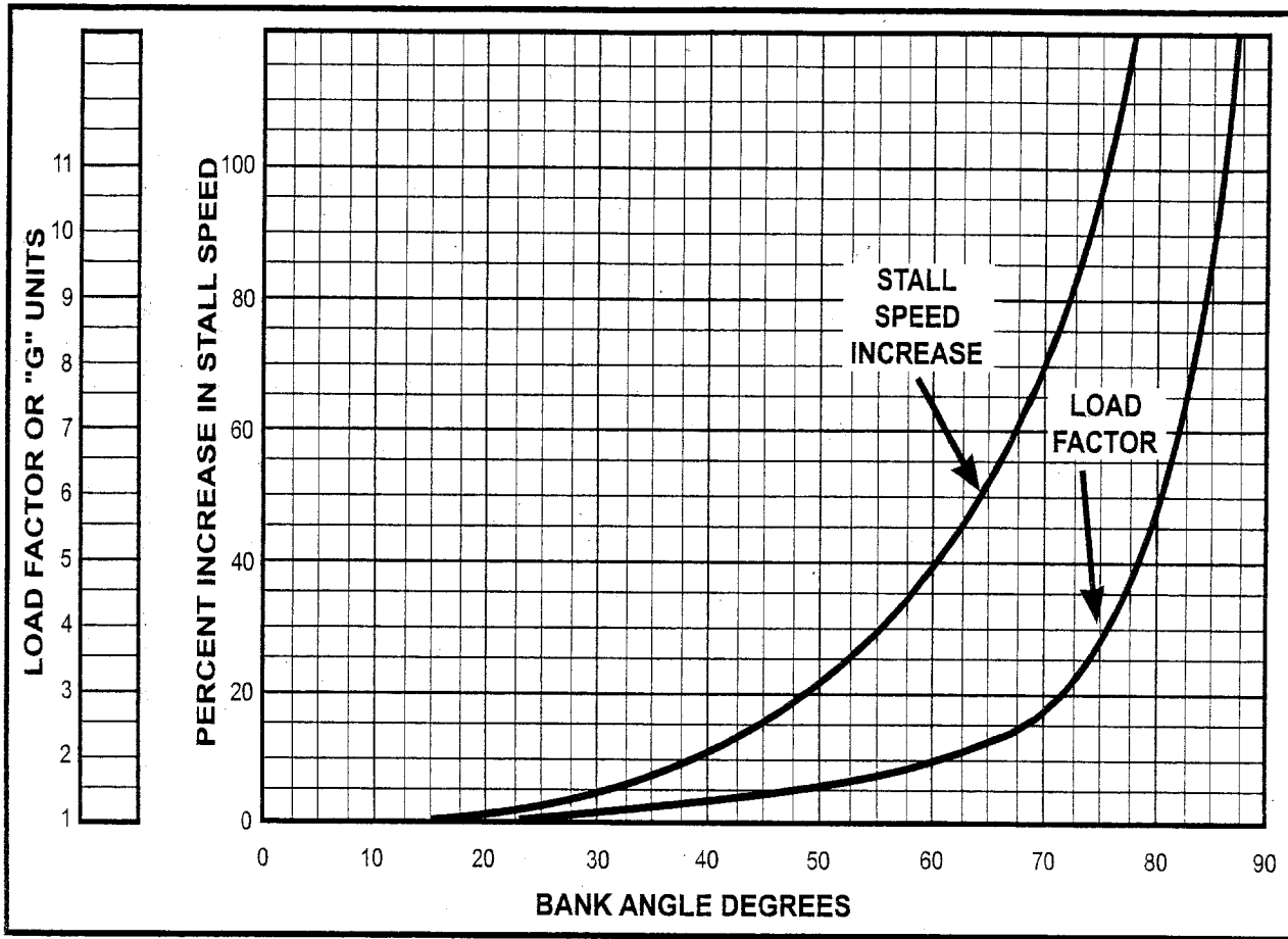
Figure 4. - Stall Speed/Load Factor.
