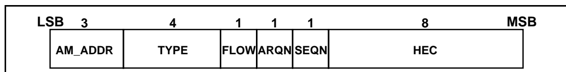
Figure 4.5: Header format.
