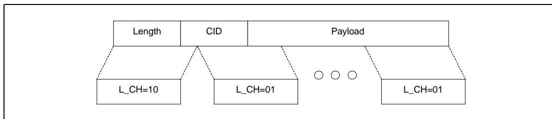
Figure 2.4: L2CAP segmentation
