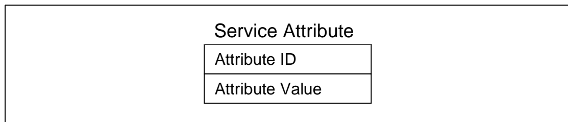
Figure 2.4: Service Attribute
