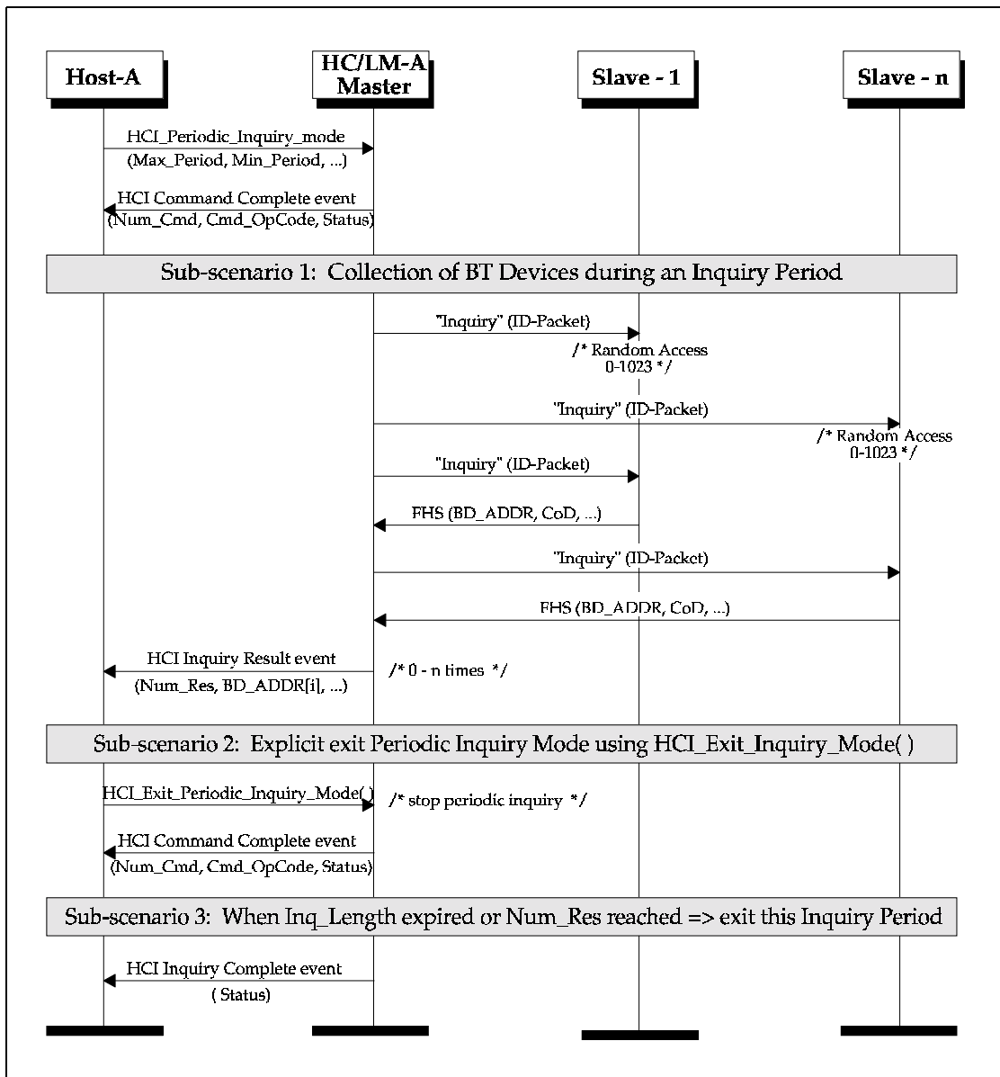
Figure 2.3: Periodic Inquiry
